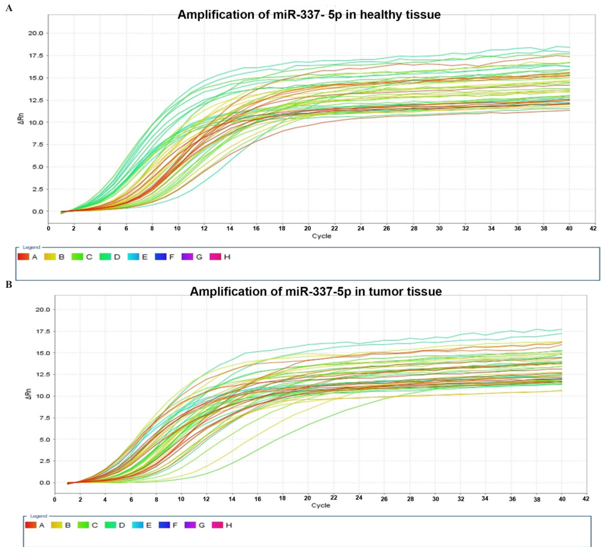
Supplementary Fig. 2. Real-time PCR amplification curve of miRNA 337-5p in (A) healthy bladder tissue samples and (B) tumour bladder tissue samples.
