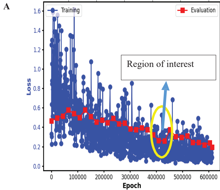
Supplementary Fig. 5. Training and evaluation loss curves.
