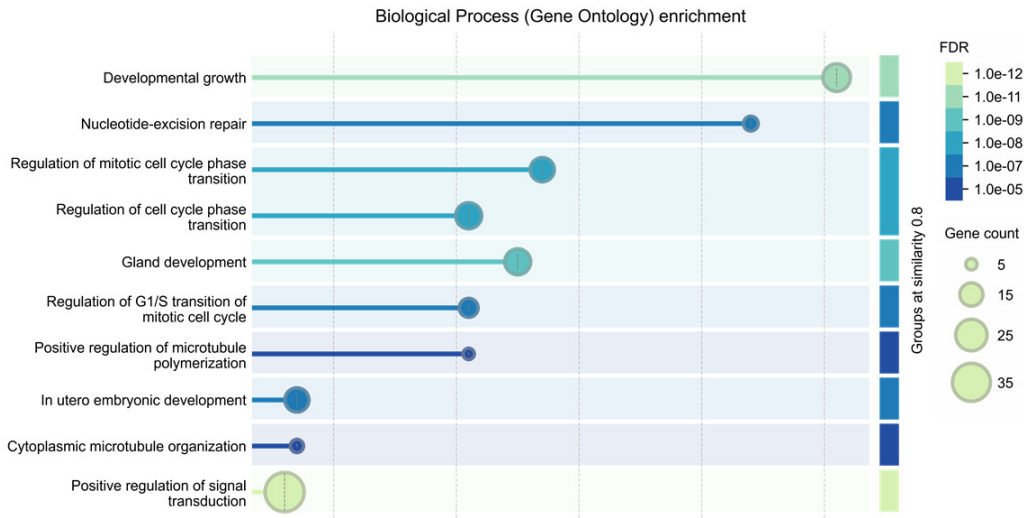
Supplementary Fig. 4D. STRINGdb ( https://string-db.org/ ) analysis for biological process gene ontologies for Basal-like subtype.
