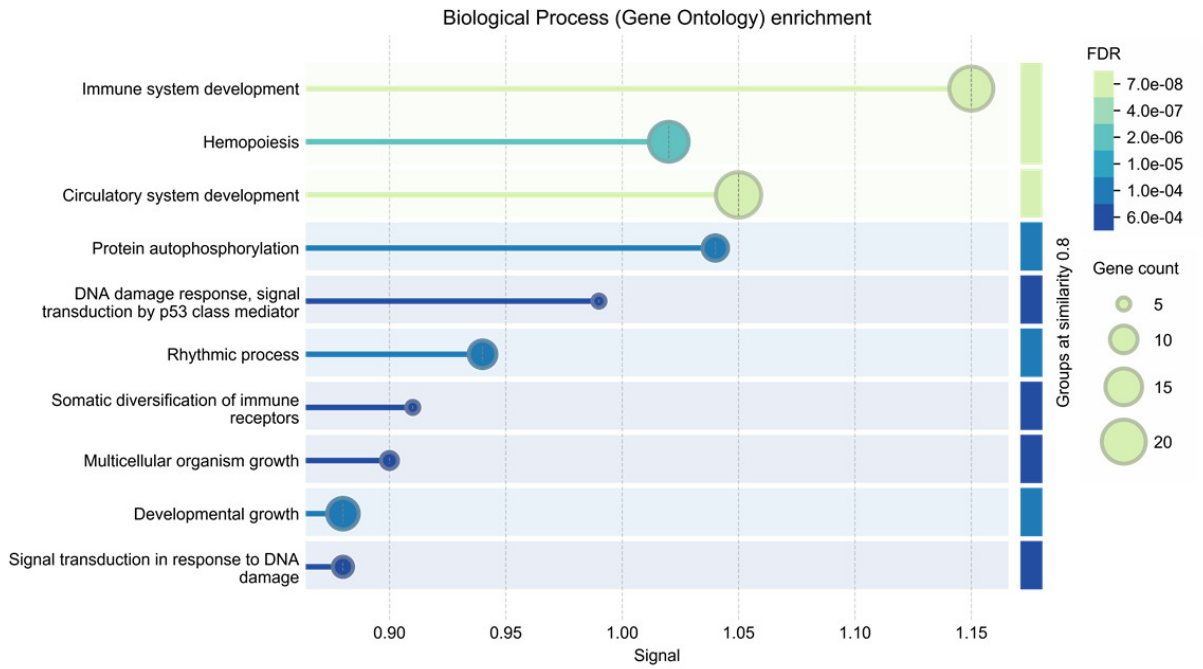
Supplementary Fig. 4A. STRINGdb ( https://string-db.org/ ) analysis for biological process gene ontologies for Luminal A subtype.
