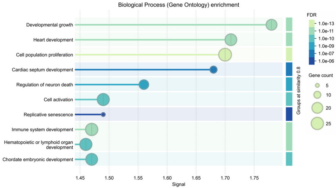
Supplementary Fig. 4B. STRINGdb ( https://string-db.org/ ) analysis for biological process gene ontologies for Luminal B subtype.
