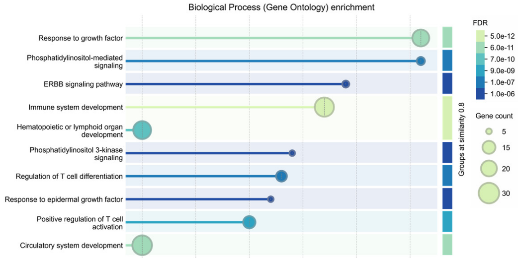
Supplementary Fig. 4C. STRINGdb ( https://string-db.org/ ) analysis for Biological Process Gene Ontologies for HER2-like subtype.
