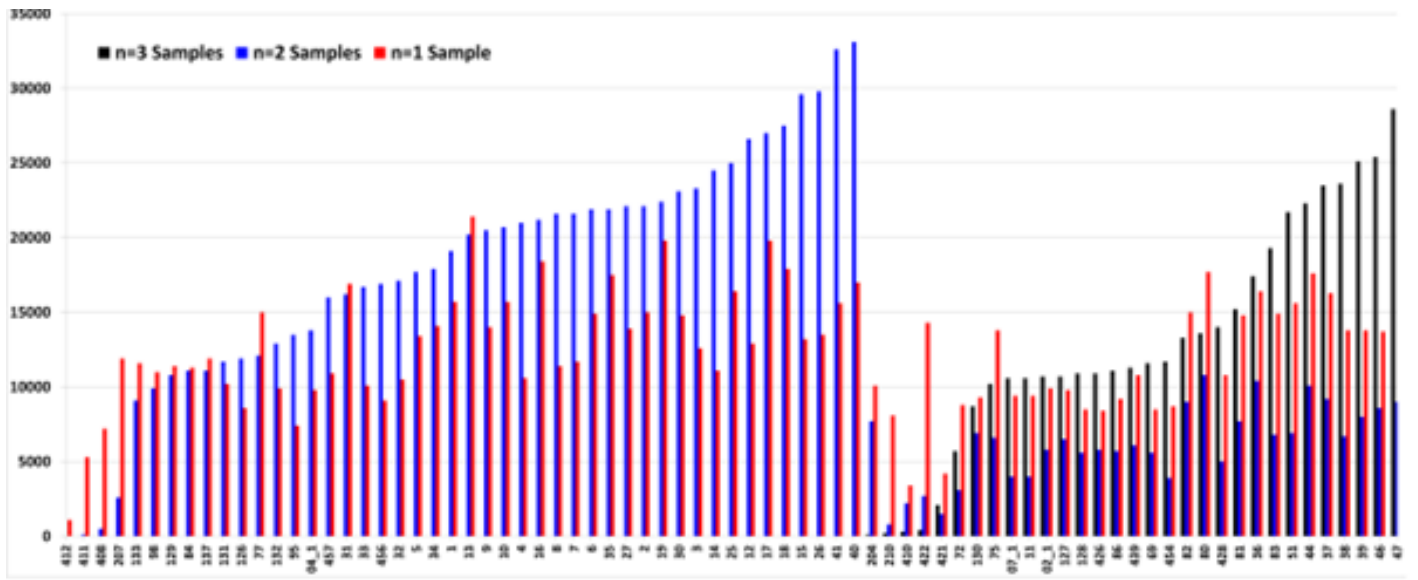
Supplementary Fig. 1. Transcript distribution across 207 samples from 97 patients.
