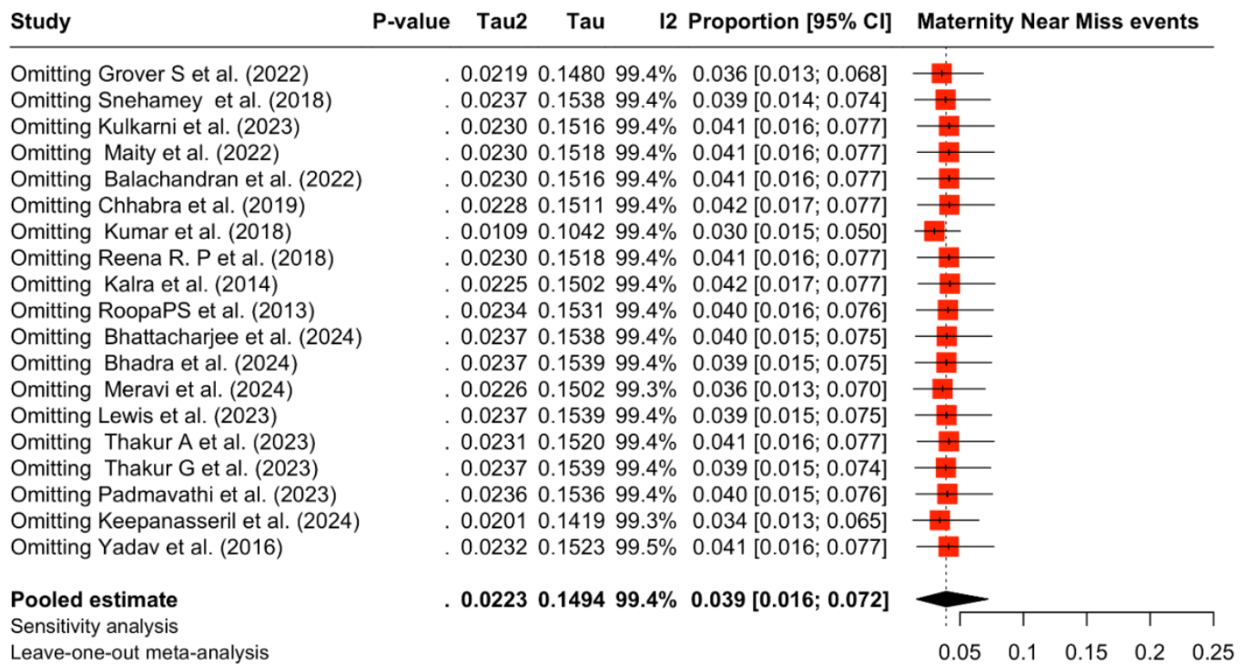
Supplementary Fig. 1. Leave one out analysis for prevalence of maternity near miss.
