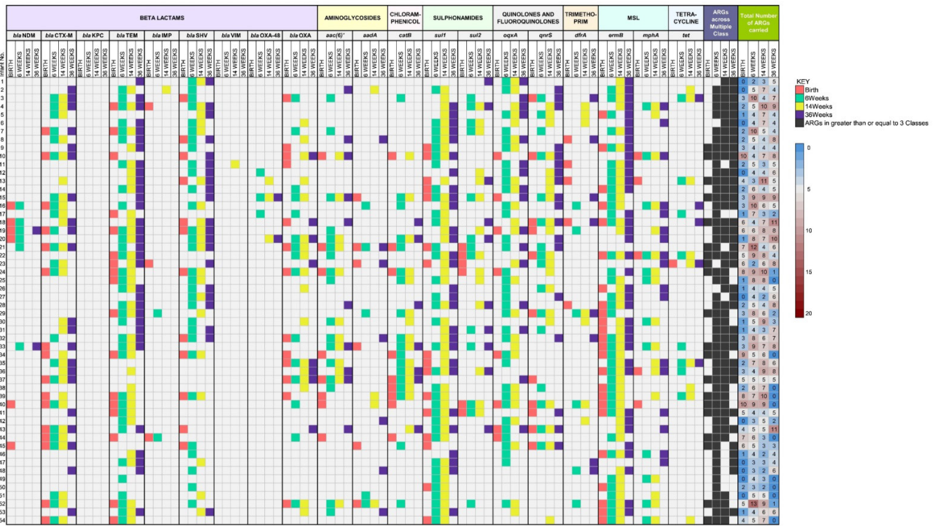
Supplementary Fig. 1. A heatmap depicting the presence of genes in infants. The genes have been categorised into respective classes. The presence of genes is marked by pink (birth), teal (6 wk), yellow (14 wk) and purple (36 wk). The dark grey boxes indicate infants carrying genes across multiple classes at a particular time point. The last column is a colour scale that indicates the number of genes carried by an infant at a given time point.
