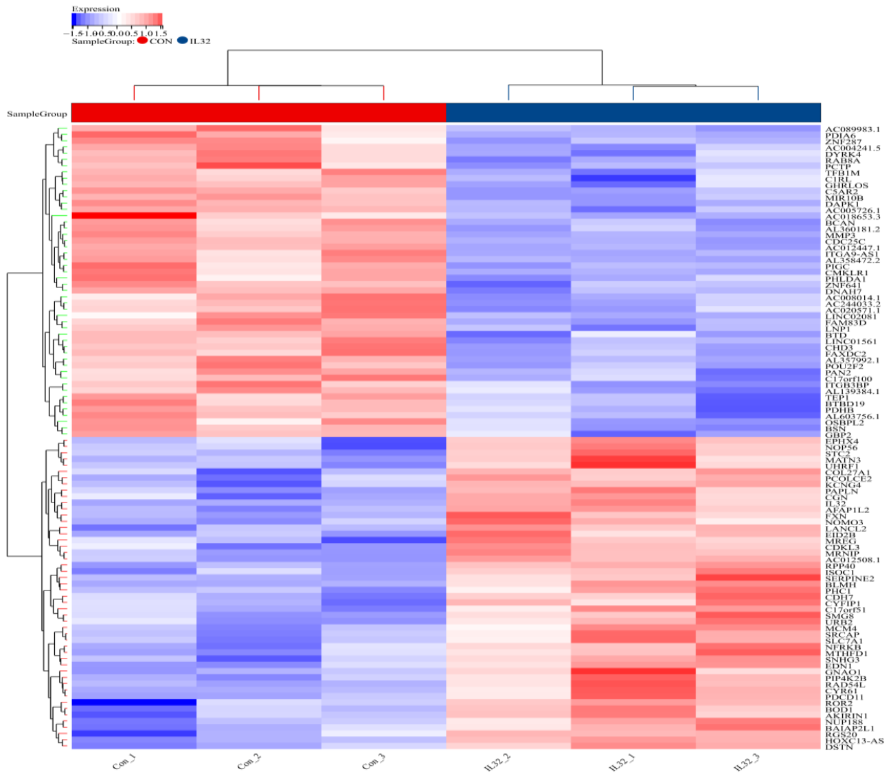
Supplementary Fig. 3. RNA sequence analysis.
