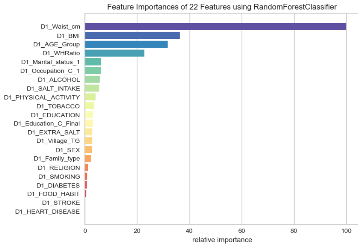
Supplementary Fig. 4. Relative Importance of the selected feature in identification of hypertension.
