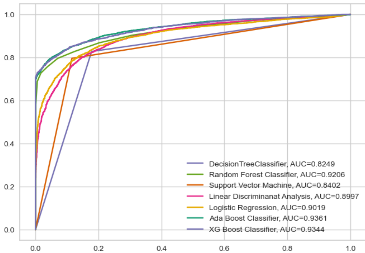
Supplementary Fig. 3. Combined ROC curves for each of the models.
