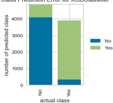
Class Prediction Error for XGBClassifier
