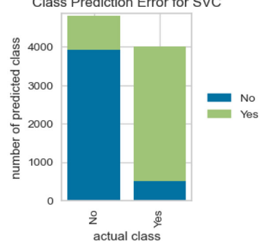
Class Prediction Error for SVC
