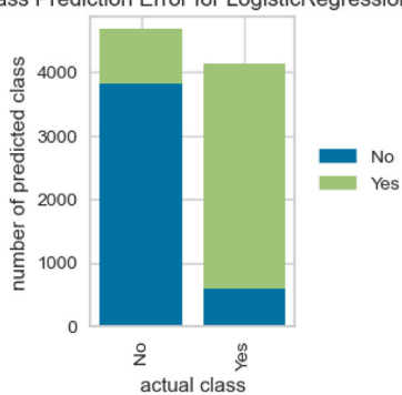
Class Prediction Error for LogisticRegression
