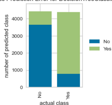
Class Prediction Error for DecisionTreeClassifier
