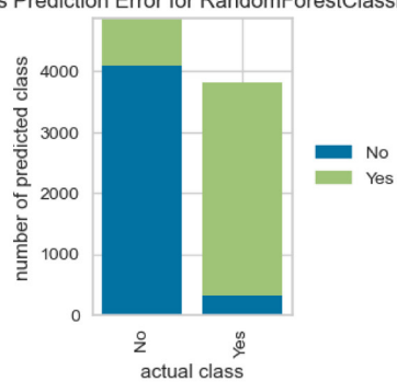
Class Prediction Error for RandomForestClassifier
