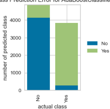
Supplementary Fig. 2. Class prediction error for each of the Models for specific randomly selected test sample in identification of hypertension.
