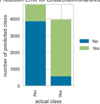
Class Prediction Error for LinearDiscriminantAnalysis
