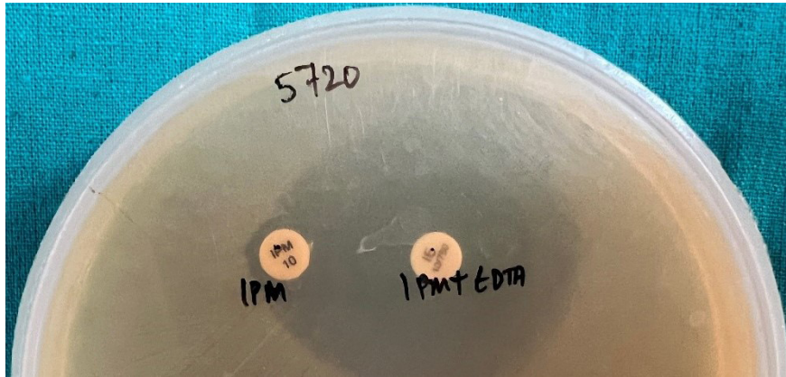
Supplementary Fig. 4. Representative image depicting positive Metallo \beta -Lactamase (MBL) production by combined-disc synergy test with 0.1 M ethylene diamine tetra acetic acid (CDST- 0.1 M EDTA).
