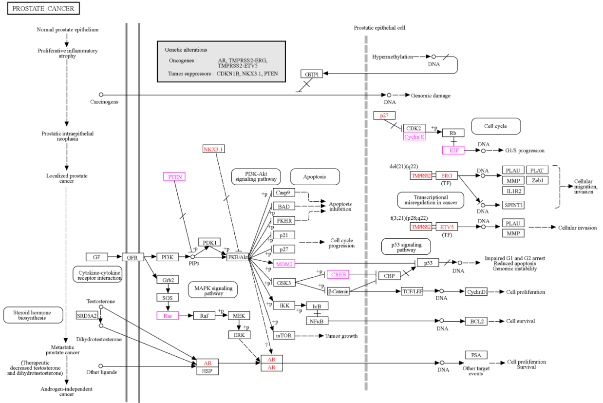
Supplementary Fig. 1. (A) The Venn diagram of the common target genes of miR-363. (B) The KEGG pathway of prostate cancer showing target genes viz., CCNE2 , PTEN , MDM2 , E2F3 and NRAS . KEGG, Kyoto encyclopedia of genes and genomes.
