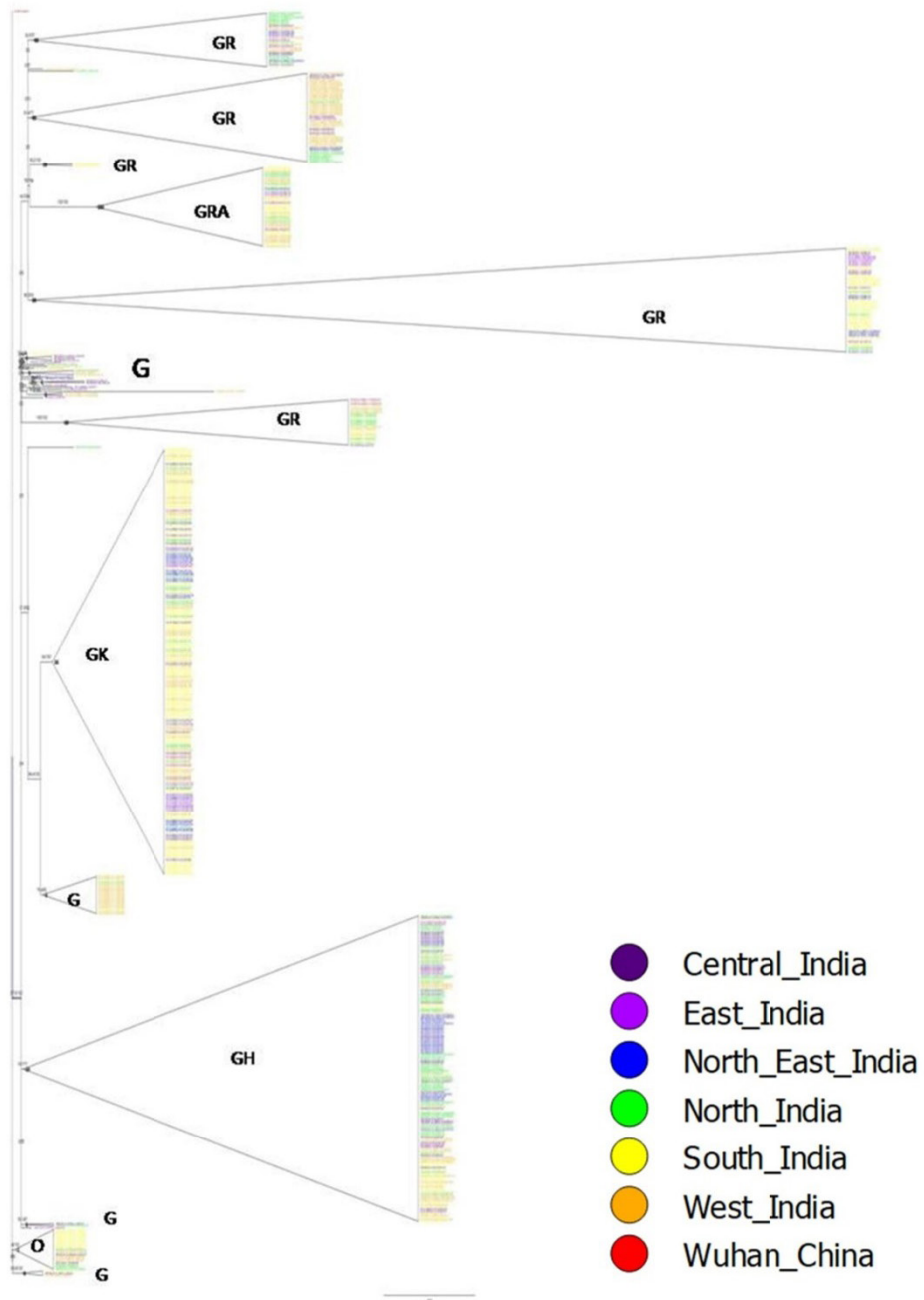
Supplementary Fig 7. Maximum likelihood tree showing the distribution of individual SARS-CoV-2 genome sequences in this study. Taxa are colored based on geographical regions of India. Nodes with >70per cent bootstrap support are labeled with corresponding clades.
