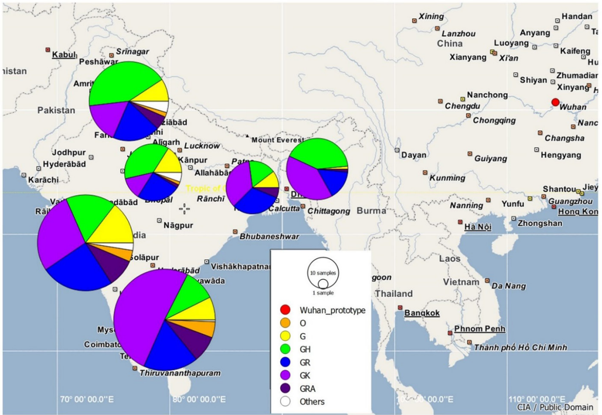
Supplementary Fig. 6. Geographical distribution of various SARS-CoV-2 clades in India. O, G, GH, GK, GR, GRA: SARS-CoV-2 clades. Source: PopART v.1.7 ( https://popart.maths.otago.ac.nz/ ).
