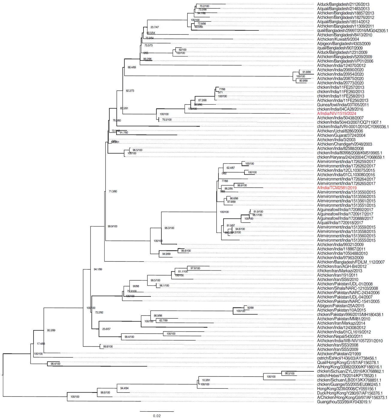
Fig. 1. Phylogenetic tree of haemagglutinin gene of A(H9N2) influenza virus from India (coloured) and reference strains. The numbers above the branches are the aLRT likelihood and ultra-bootstrap probabilities (%) for each branch, respectively determined by using IQTREE. The previously reported sample from India is highlighted. Scale bars indicate nucleotide substitutions per site.
