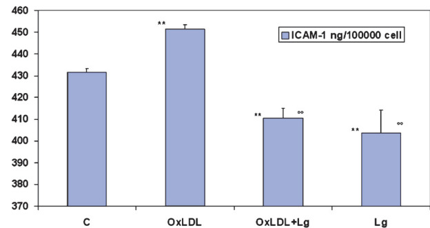
Fig. 2. Effect of oxLDL on endothelial ICAM-1 production. Lisosan G shows a significant reduction of ICAM-1 medium concentration (ELISA method). ** P<0.01 compared to control; °° P<0.01 compared to ox-LDL incubation.
