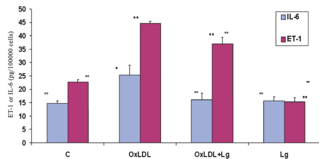
Fig. 3. Effect of ox-LDL on endothelial IL-6 and ET-1 production. These markers were significantly reduced after the incubation with Lisosan G. * P<0.05 , ** P<0.01 compared to control; °° P<0.01 compared to ox-LDL incubation.
